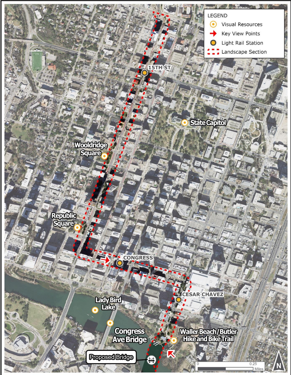
Figure 5: Downtown Section
