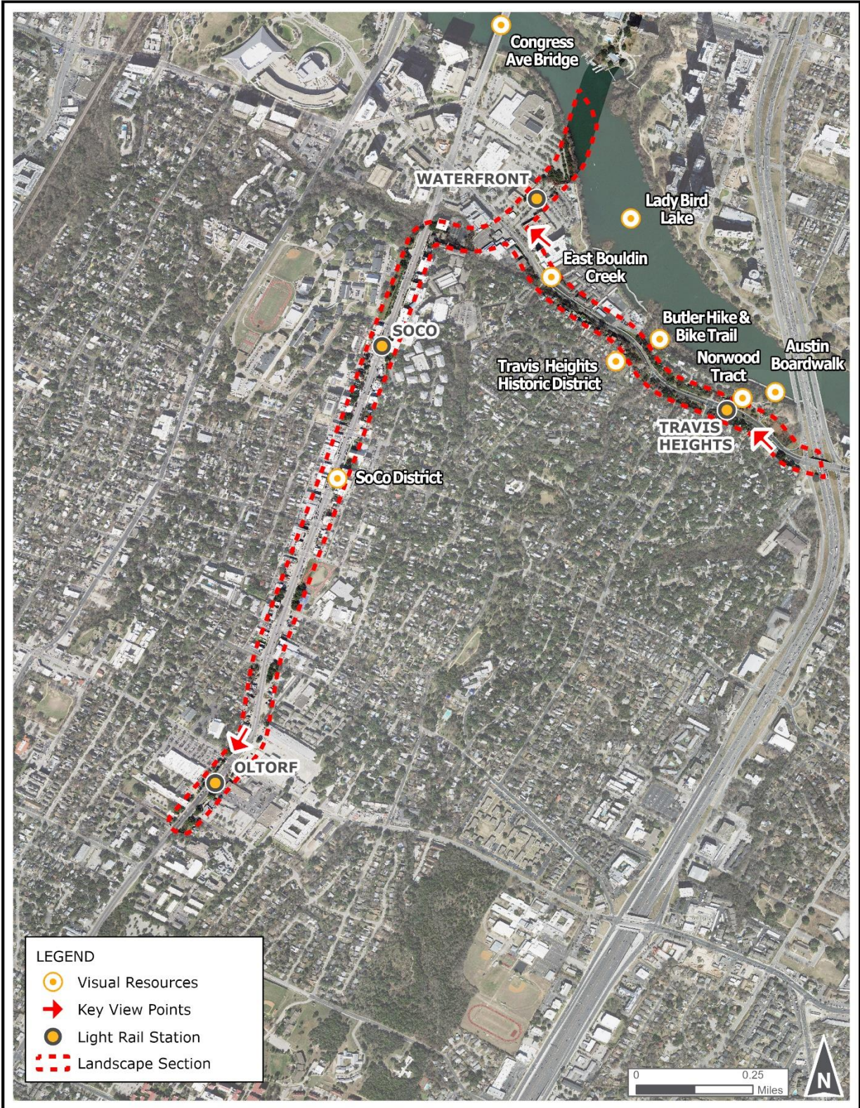
Figure 7: South Section
